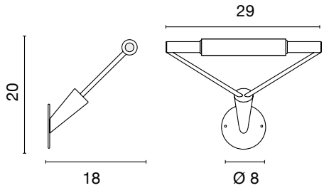
4138 1 kg 160W R7s ECO F IP 40 .22 .32
