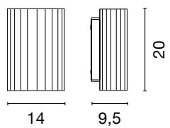
4265 1,4 kg 120W R7s (78 mm.) ECO F .50
