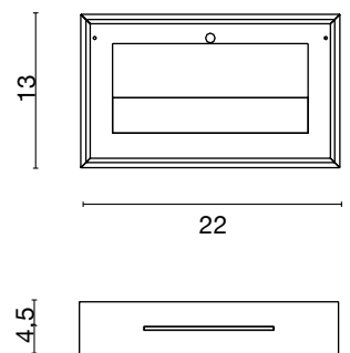
4321 1,1 kg 120W R7s (78 mm) ECO .57
